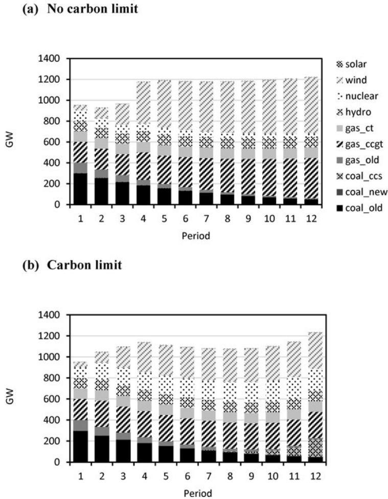
Figure 4: Optimal Installed Capacities without Power System Details Modeled
